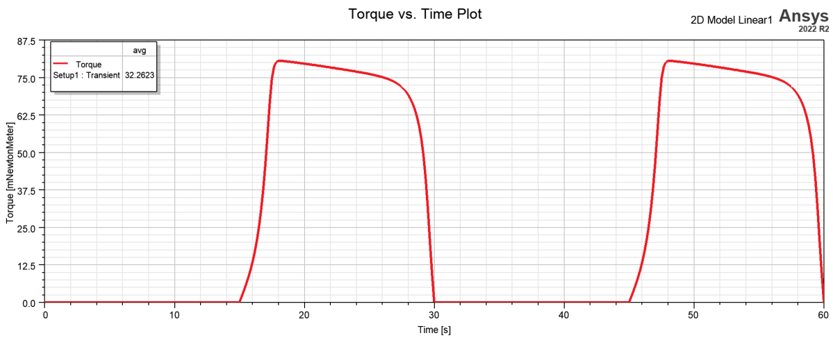
Figure 12: Torque variation with respect to time from FEA simulations with control strategy implemented.
