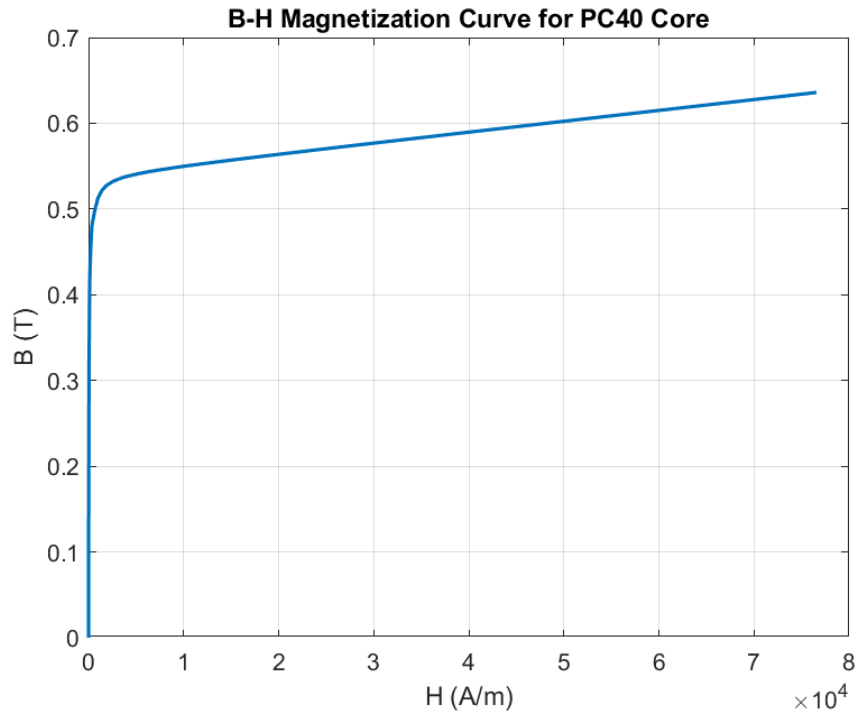
Figure 13: B-H curve of the PC40 core used in the FEA simulations.
